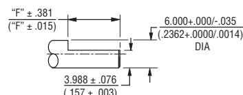
SHAFT TYPE "S" (USES BUSHING R)
