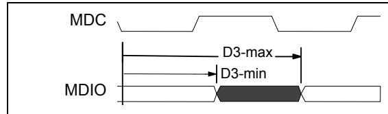
Figure 25 - MDIO Output Delay Timing
