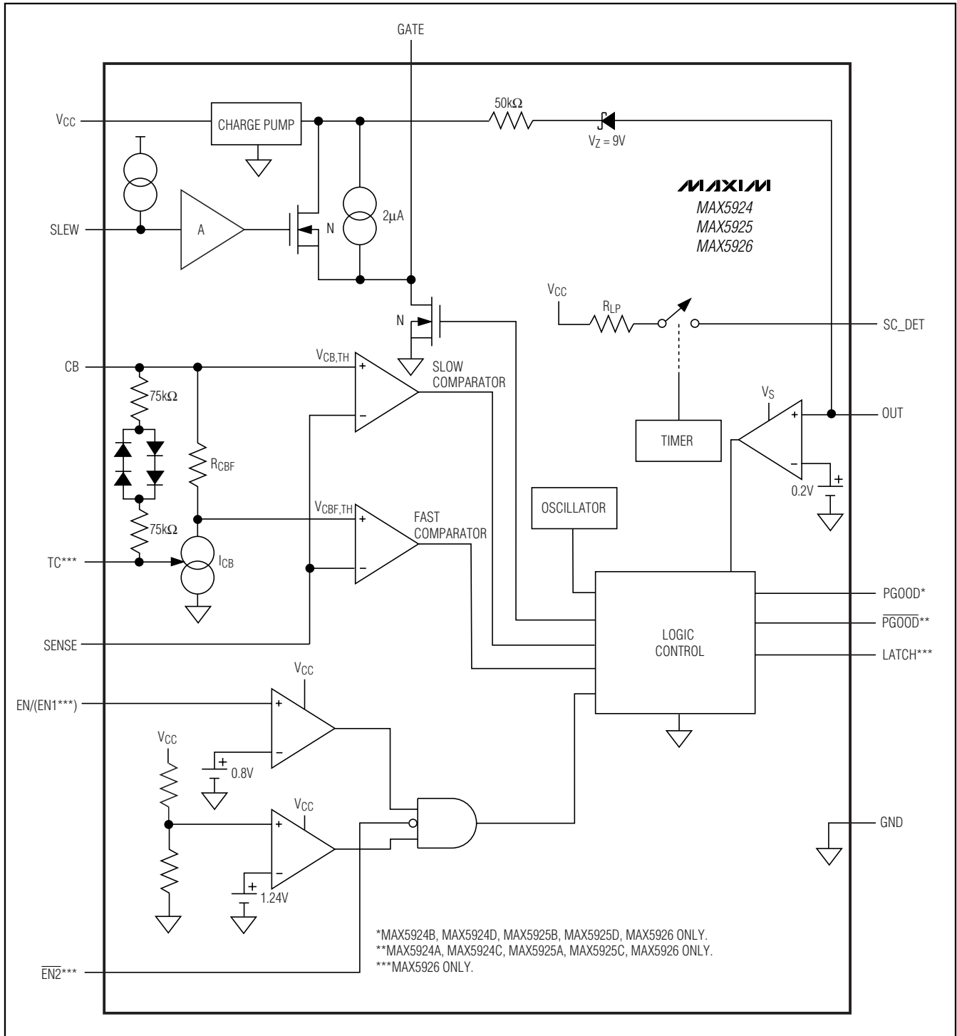
Figure 3. Functional Diagram
