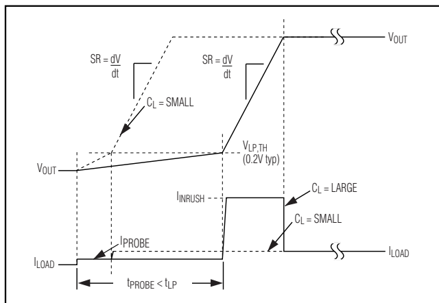
Figure 5. Startup Waveform
