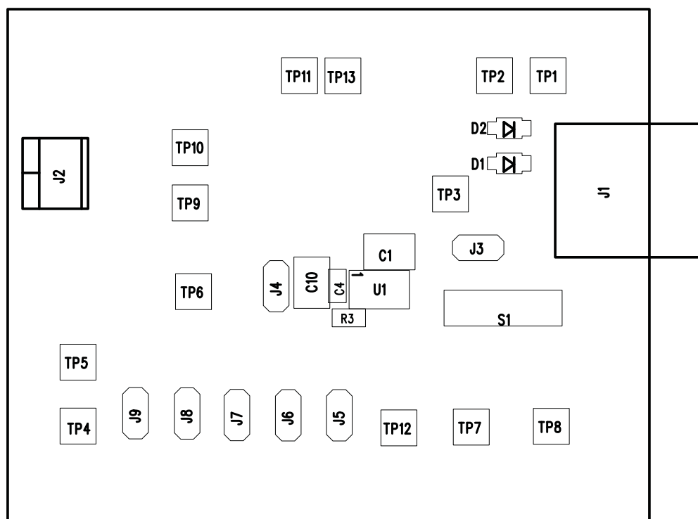
Figure 4. TPS2511EVM-141 Layer 1
