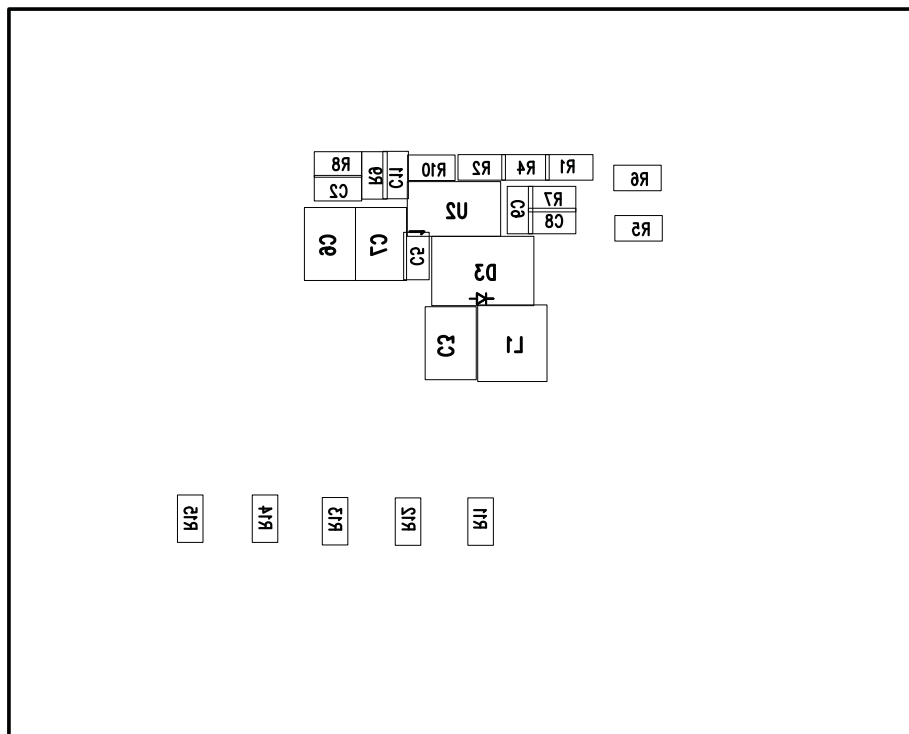
Figure 8. Bottom Layer
