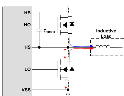
Figure 24. Parasitic Inductance on HS Node
