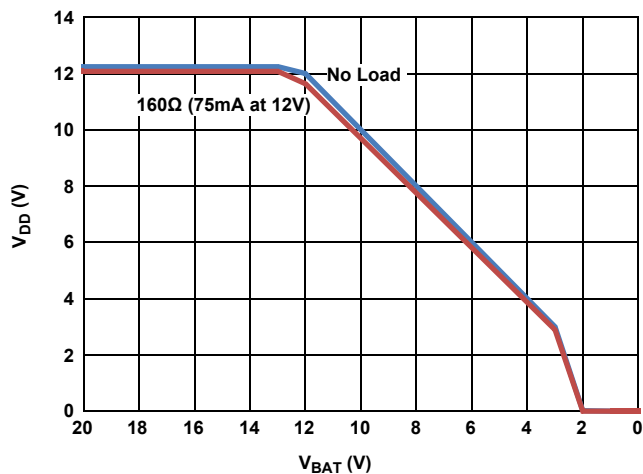
Figure 10. V_{DD} Dropout vs V_{BAT} (HIP2104 Only)
