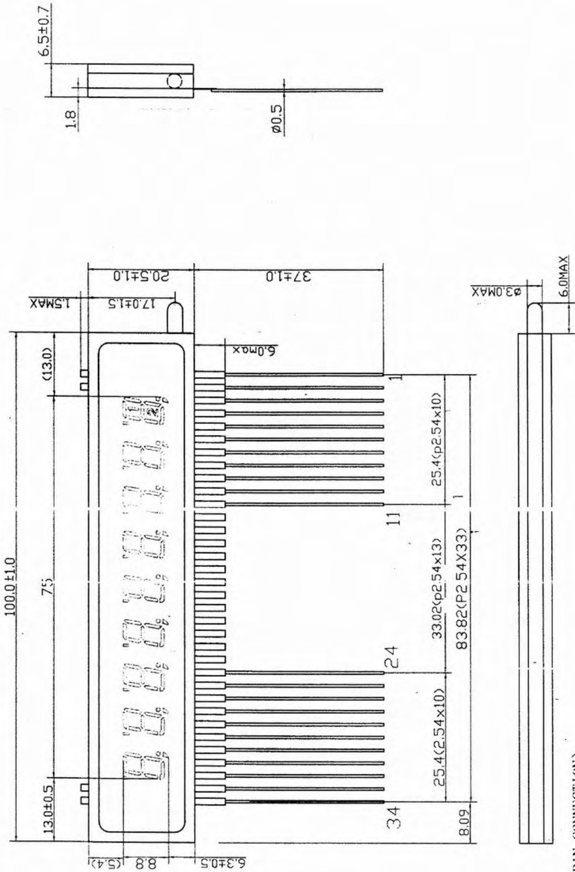
外形图(OUTER DIMENSION) (UNIT IN mm)
