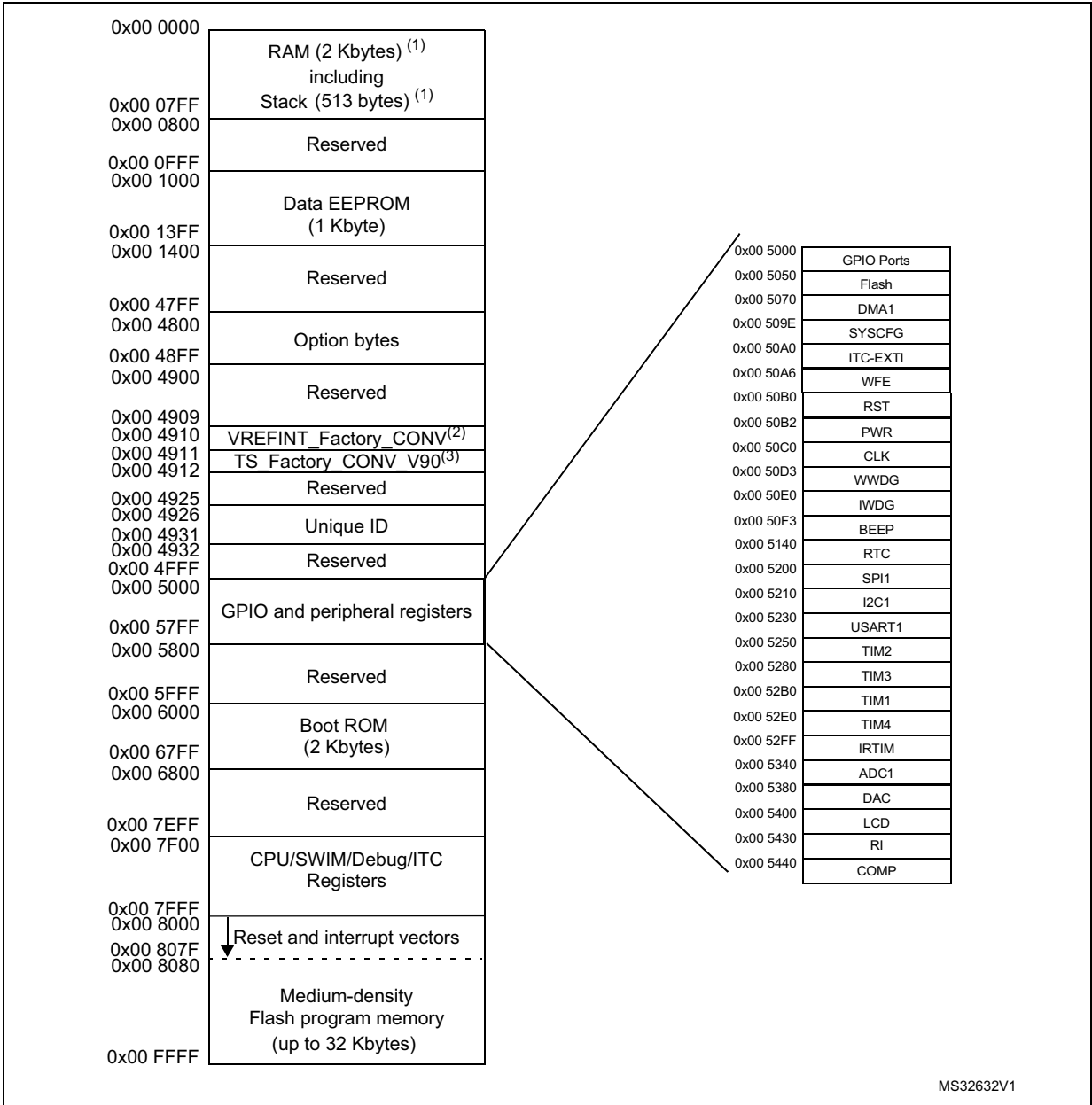
Figure 9. Memory map
