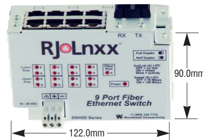
Part Number Description ENHSDURS9 Ethernet Switch, 8 x RJ-45 Ports 1 x Duplex SC Port
