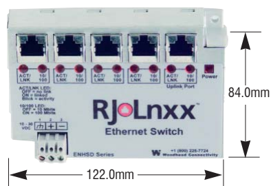
Part Number Description ENHSDURR5 Ethernet Switch, 5 x RJ-45 Ports
