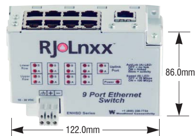
Part Number Description ENHSDURR9 Ethernet Switch, 9 x RJ-45 Ports
