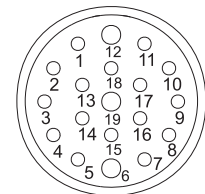
Female insert on plug side
