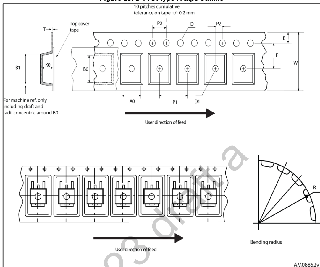
Figure 13: D 2 PAK type A tape outline
