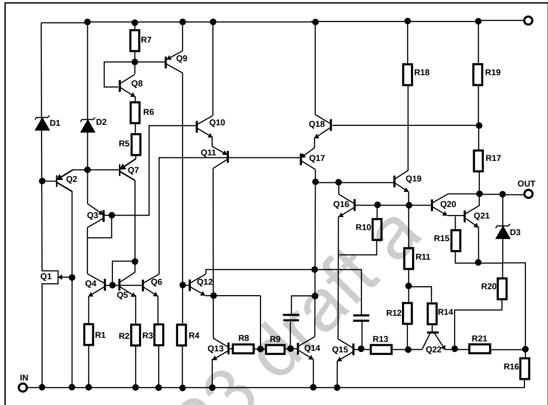
Figure 1: Schematic diagram
