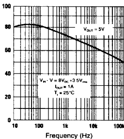
RIPPLE REJECTION
