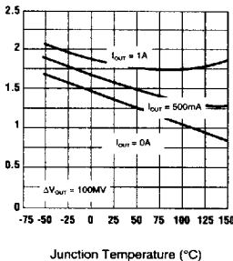
DROPOUT VOLTAGE
