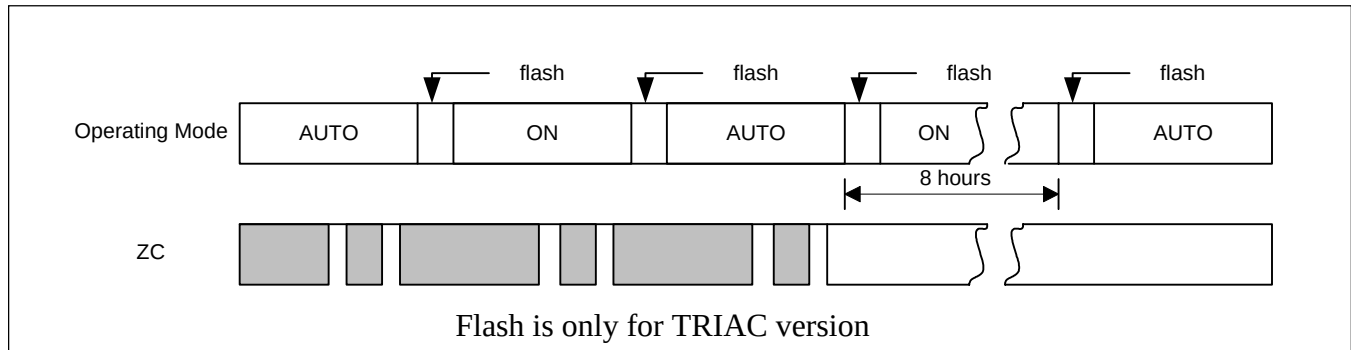
Figure 7. Override Timing
