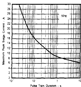
Fig. 4 - Non-Repetitive Surge Ratings
