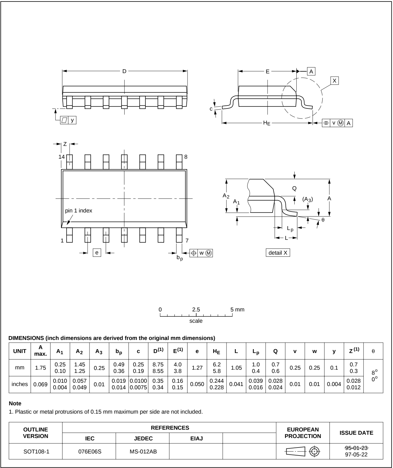
SO14: plastic small outline package; 14 leads; body width 3.9 mm
