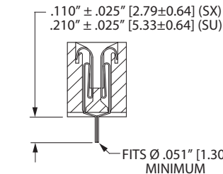
CENTERED DIP SOLDER (SX, SU) AVAILABLE WITH DUAL OR HALF LOADED READOUT TYPE
