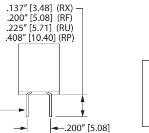
WIDE DIP SOLDER (RF, RX, RU, RP)
