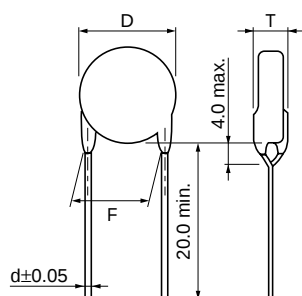
Note: Tolerance of Lead Space
