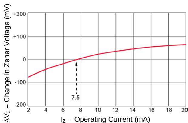
FIGURE 3 TYPICAL CHANGE OF ZENER VOLTAGE WITH CHANGE IN OPERATING CURRENT
