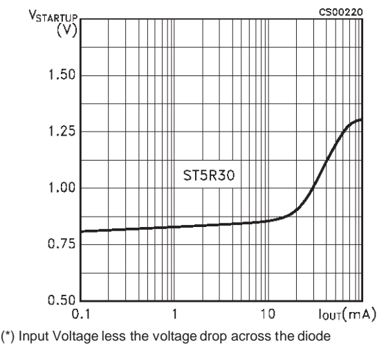
Figure 20: Minimum Input Voltage vs Output Current
