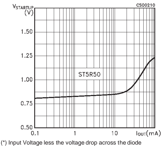
Figure 19: Minimum Input Voltage vs Output Current
