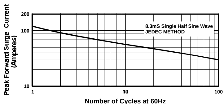
FIGURE 6. MAXIMUM NON-REPETITIVE PEAK FORWARD SURGE CURRENT - UNIDIRECTIONAL
