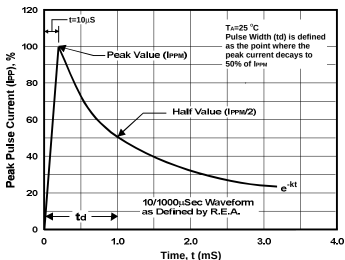
FIGURE 3. PULSE WAVEFORM
