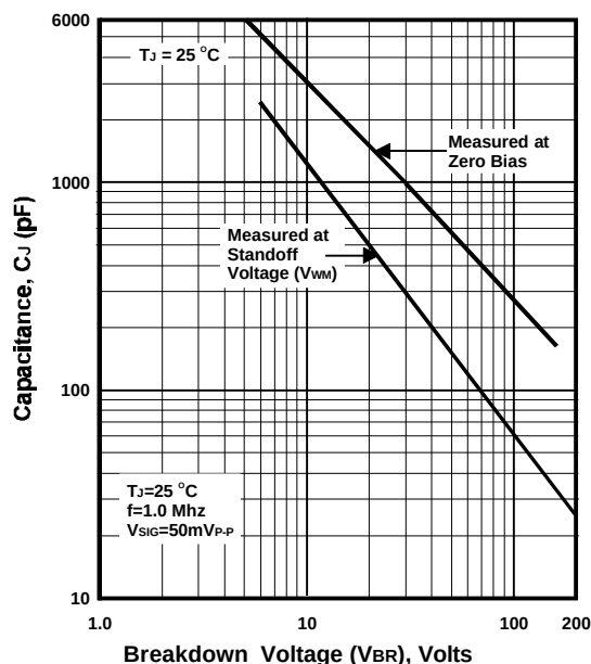
FIGURE 4. TYPICAL JUNCTION CAPACITANCE-UNIDIRECTIONAL
