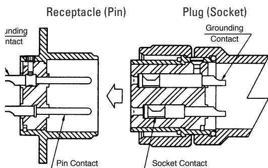
Connector Profile (Ref.)
