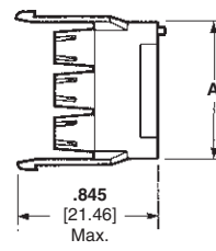
Cap Rear
