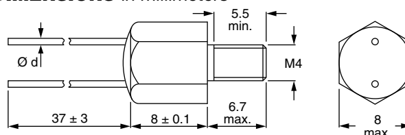
Component outline
