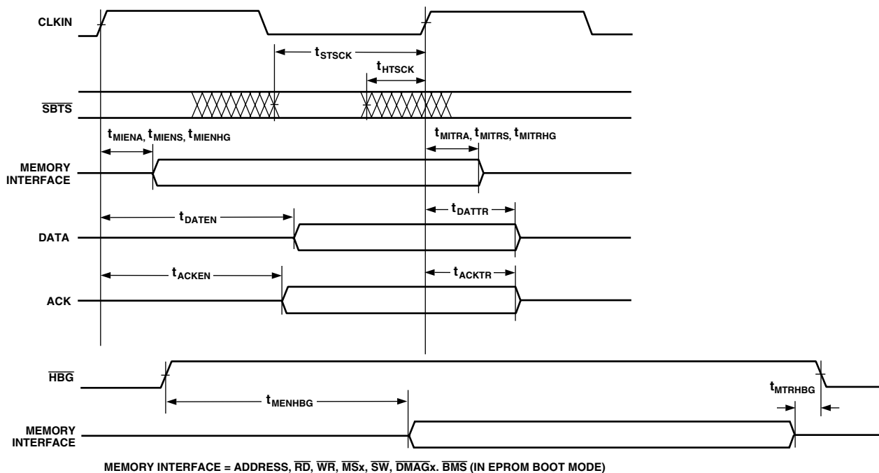
Figure 17. Three-State Timing
