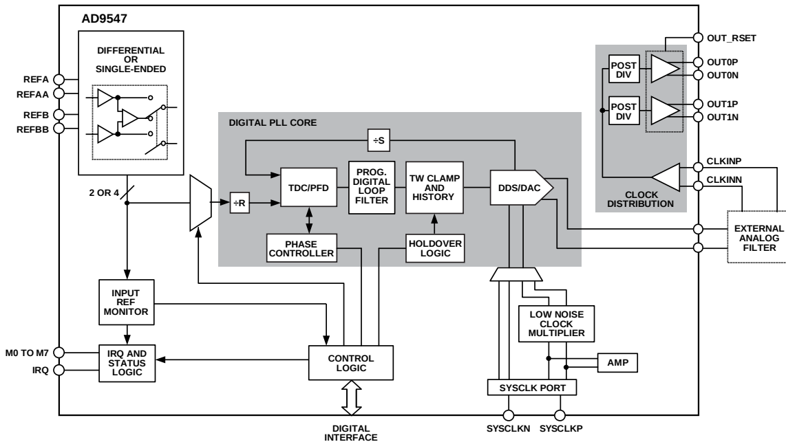
Figure 33. Detailed Block Diagram
