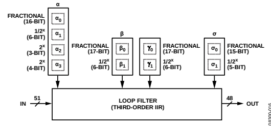
Figure 40. Third-Order Digital IIR Loop Filter
