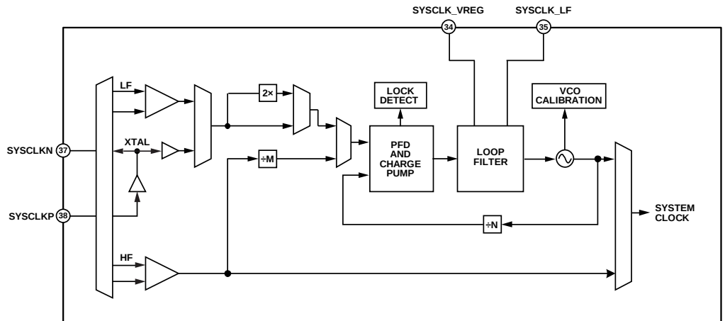
Figure 45. System Clock Block Diagram
