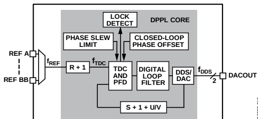
Figure 37. Digital PLL Core
