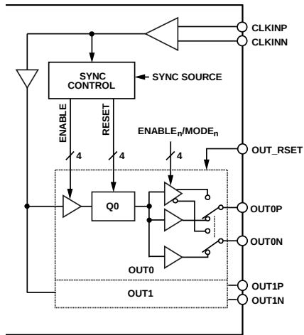
Figure 47. Clock Distribution
