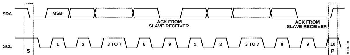
Figure 63. Data Transfer Process (Master Write Mode, 2-Byte Transfer Used for Illustration)
