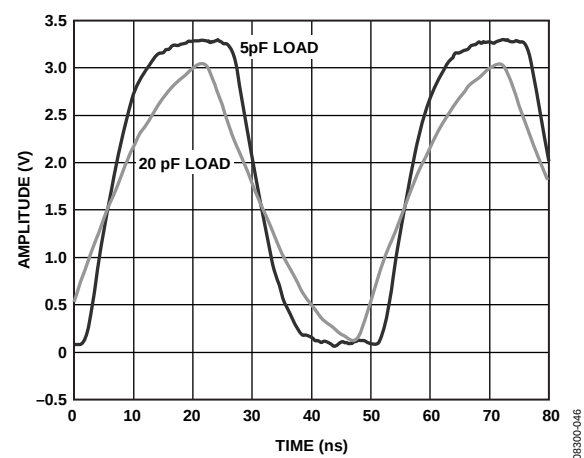
Figure 24. Output Waveform, 3.3 V CMOS (20 MHz, Weak Mode)
