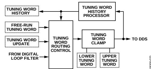
Figure 44. Tuning Word Processing
