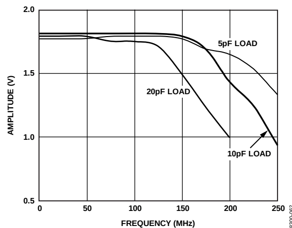
Figure 16. Amplitude vs. Toggle Rate, 1.8 V CMOS
