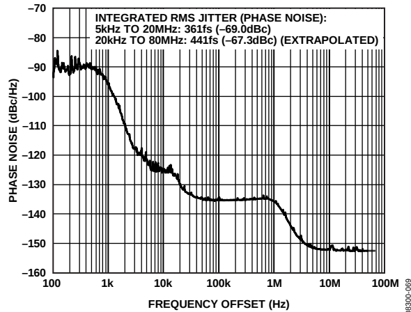
Figure 7. Additive Phase Noise (Output Driver = LVPECL), f_{REF} = 19.44 MHz, f_0 = 155.52 MHz, LBW = 1 kHz, f_{SYSCLK} = 50 MHz, PLL On
