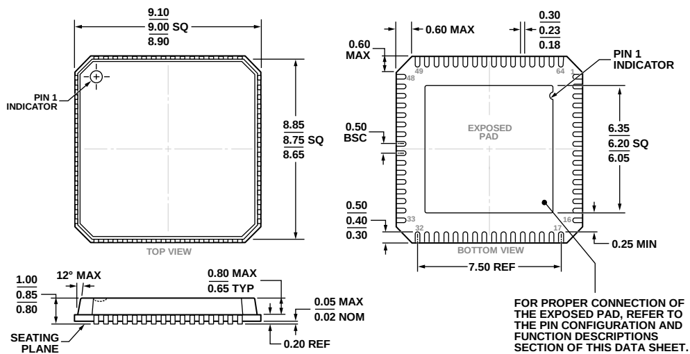
Figure 69. 64-Lead Lead Frame Chip Scale Package [LFCSP_VQ]
