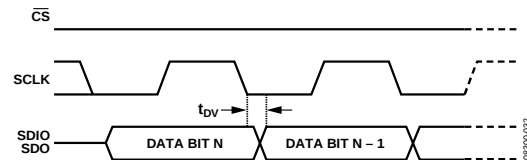
Figure 57. Serial Control Port Timing—Read
