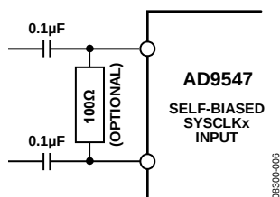
Figure 29. SYSCLKx Input
