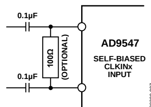
Figure 30. CLKINx Input
