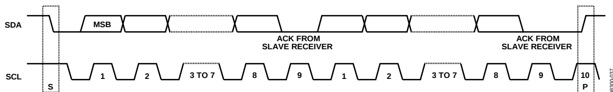
Figure 62. Acknowledge Bit
