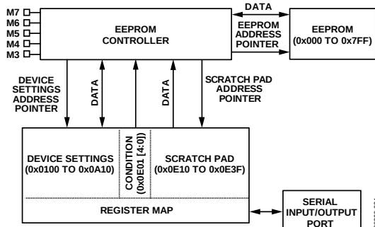
Figure 49. EEPROM Functional Diagram
