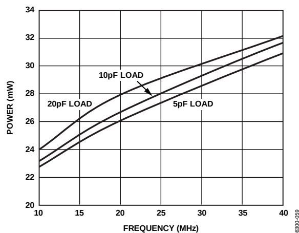
Figure 22. Power Consumption vs. Frequency, 3.3 V CMOS (Weak Mode)
