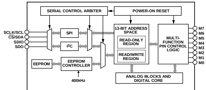
Figure 51. Serial Port Functional Diagram
