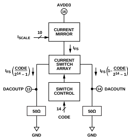
Figure 43. DAC Output Pins
