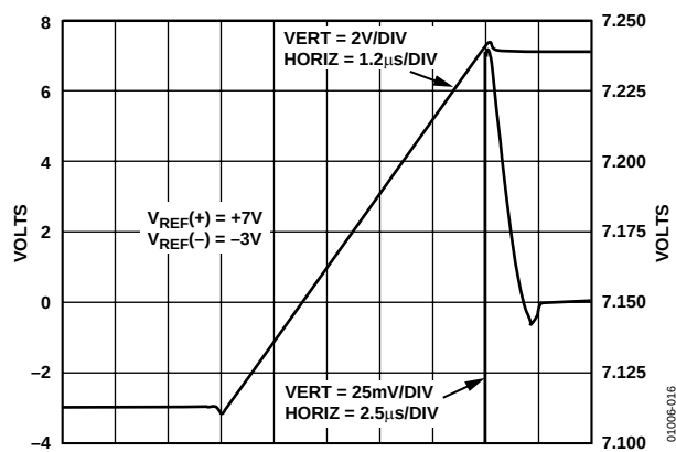
Figure 16. Settling Time (+)
