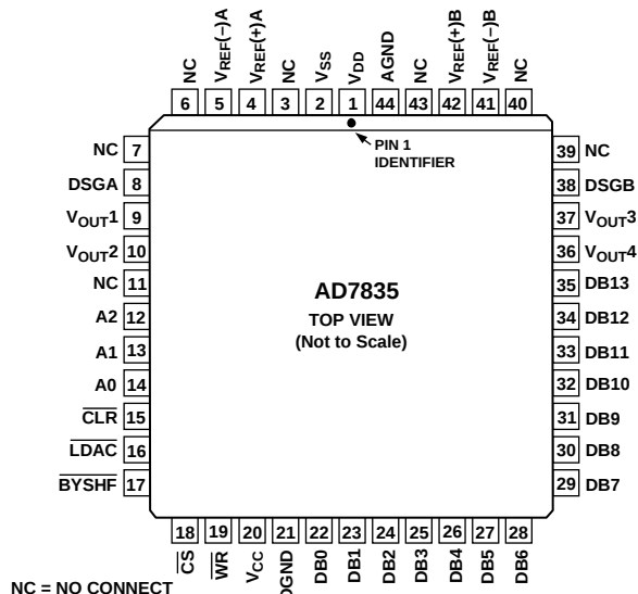
Figure 8. AD7835 PLCC
