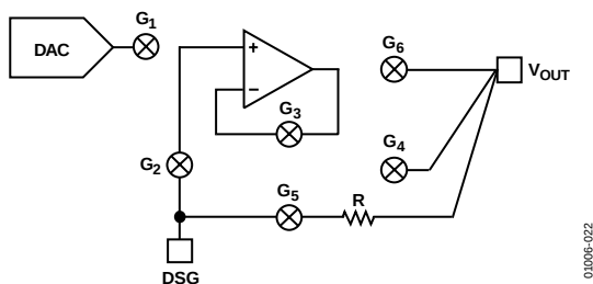
Figure 22. Output Stage with V_{DD} < 10\text{ V}
