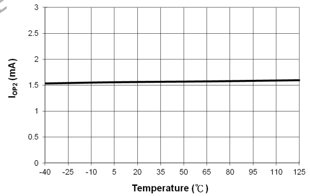
Figure 8. FSL5x8H I OP2 vs. Temperature
