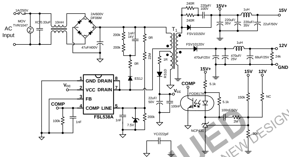
Figure 49. FSL538AFlyGEB Schematic
