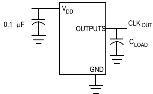
Figure 7. Test Circuit #1
