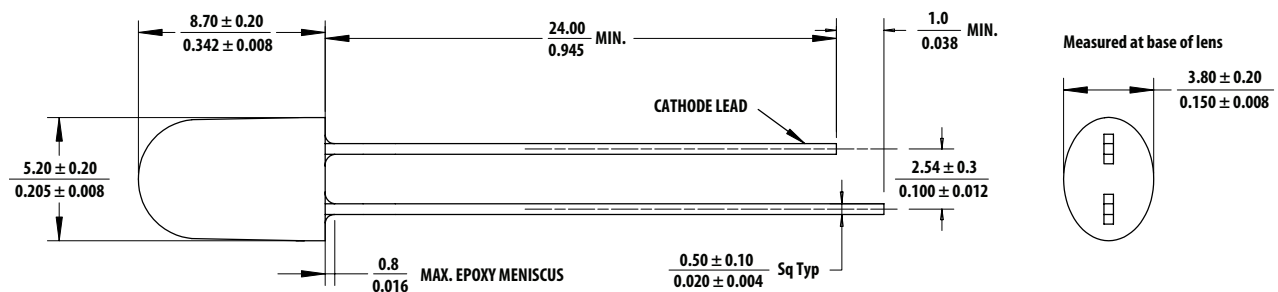
Package drawing B
