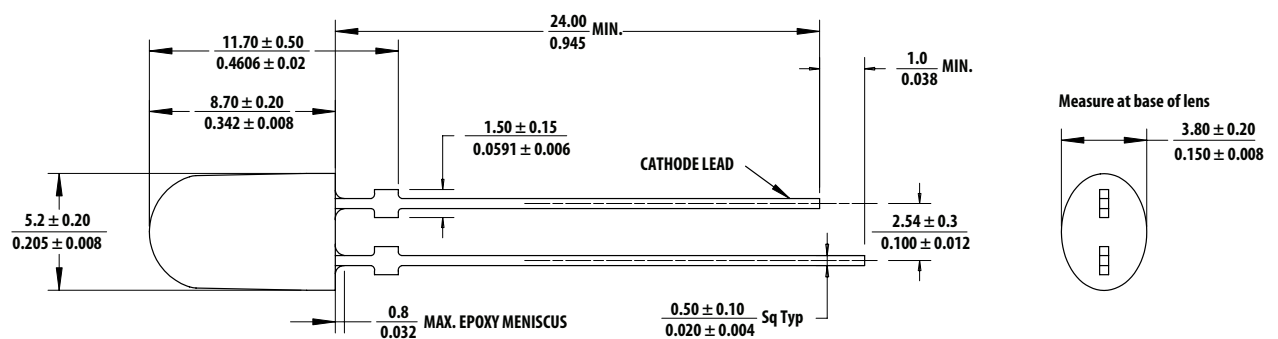
Package drawing B
