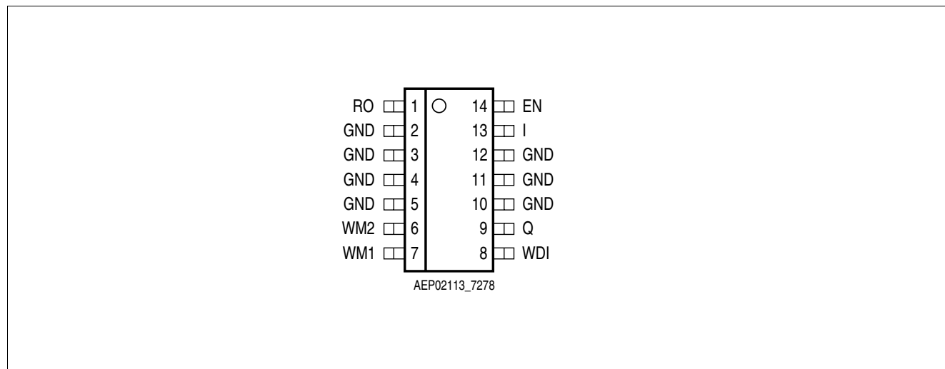
Figure 2 Pin Configuration
