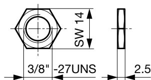
Hexagonal nut TZZ12 / TZZ51
