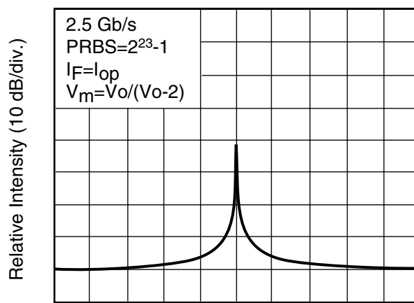
Fig. 2 Lasing Spectrum
