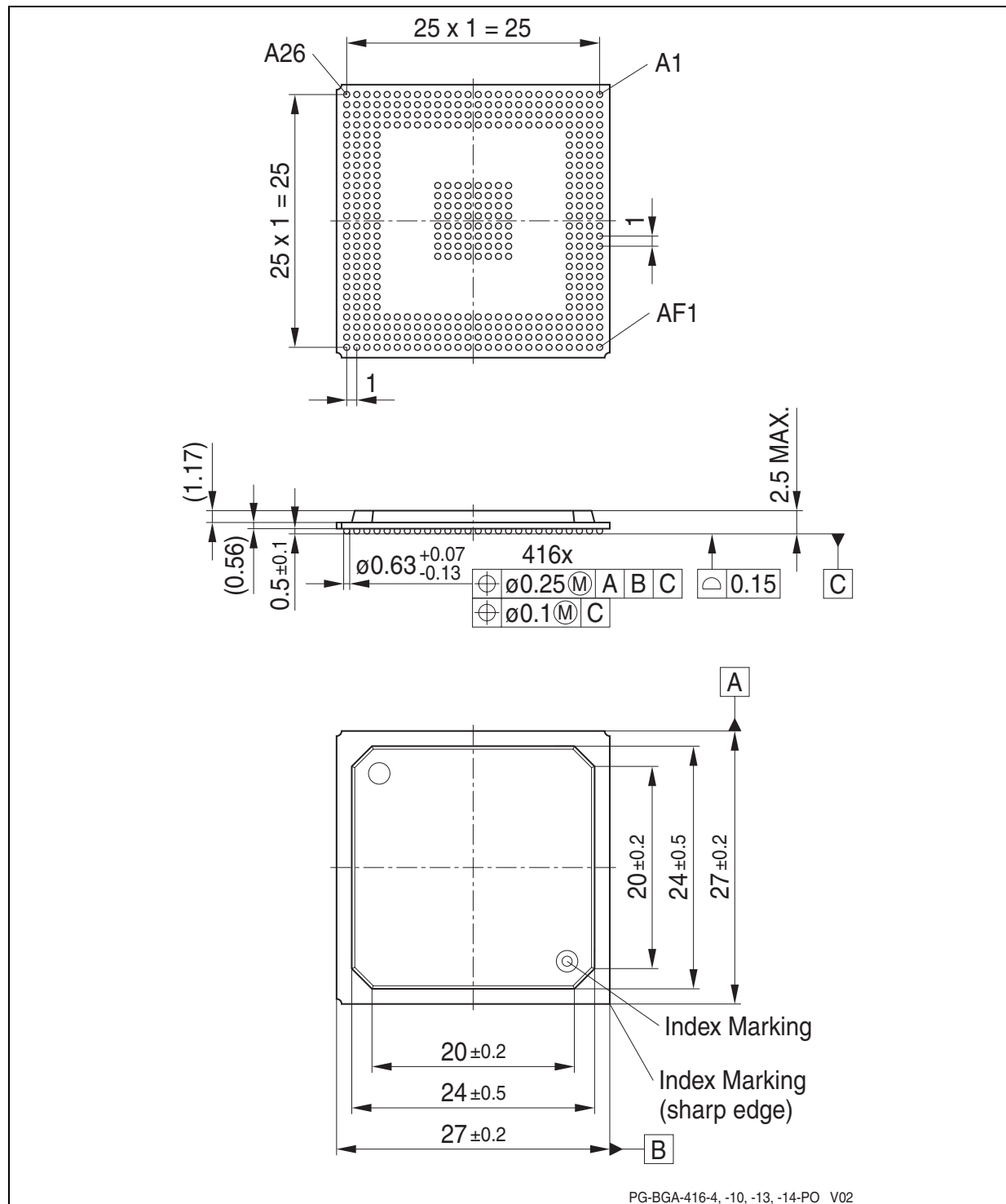
Figure 45 Package Outlines P/PG-BGA-416-10, Plastic (Green) Ball Grid Array
