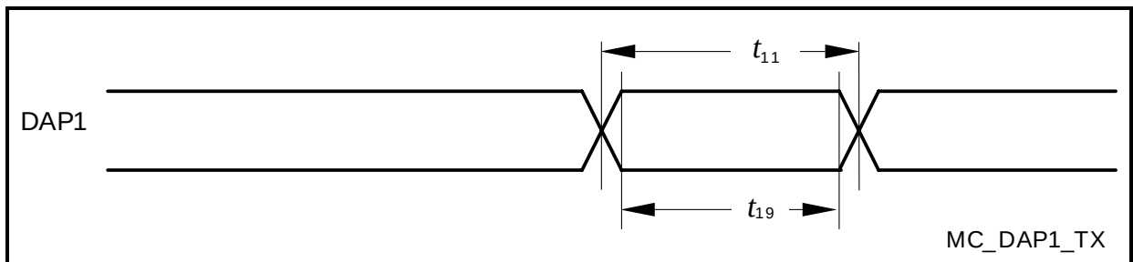
Figure 33 DAP Timing Device to Host
