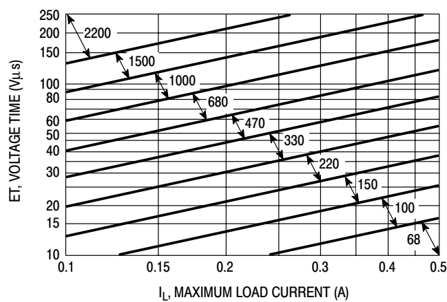
Figure 23. LM2574-ADJ
