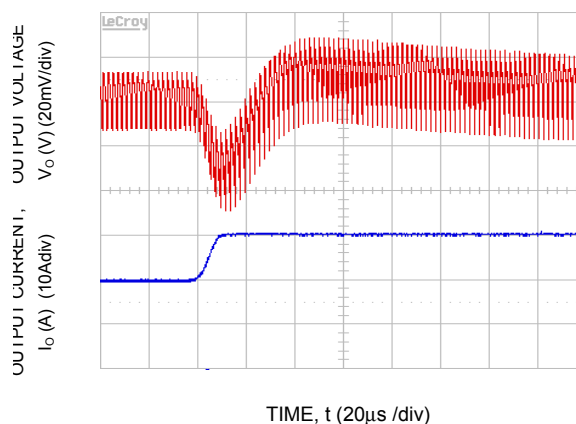
Figure 16. Transient Response to Dynamic Load Change from 50% to 100% at 12V in , C_{out} = 2x47\mu F + 3x330\mu F , C_{Tune}=5600pF & R_{Tune}=220\text{ ohms}
