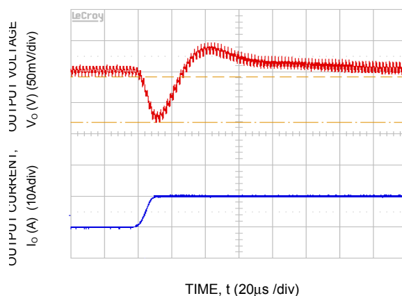
Figure 28 Transient Response to Dynamic Load Change from 50% to 100% at 12Vin, C_{out}= 5x47\mu F + 1x330\mu F , C_{Tune}=2200pF & R_{Tune}=220 ohms
