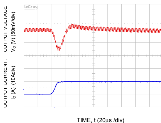
Figure 34. Transient Response to Dynamic Load Change from 50% to 100% at 12Vin, C_{out} = 8 \times 47\mu\text{F} , C_{Tune}=1500\text{pF} & R_{Tune}=220\text{ ohms}
