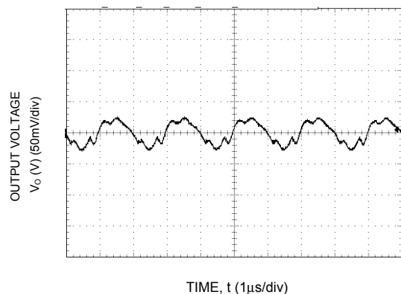
Figure 27. Typical output ripple and noise ( C_o=2x47\mu F ceramic, V_{in} = 12V , I_o = I_{o,max} ).
