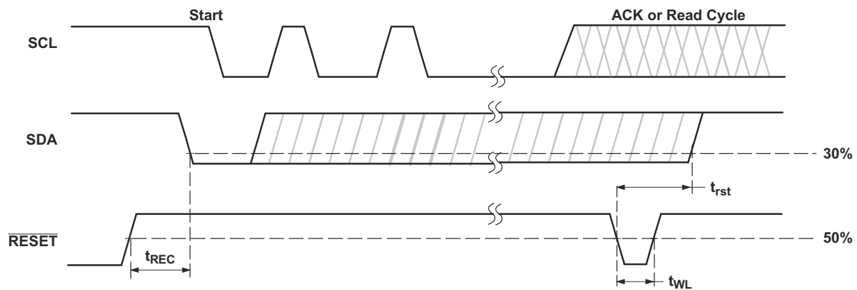
Figure 7-2. Reset Timing
