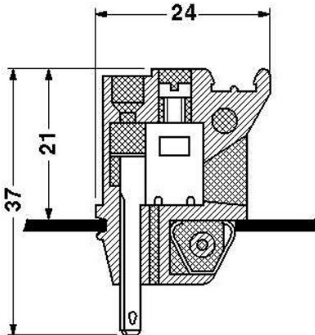
Dimensioned drawing
