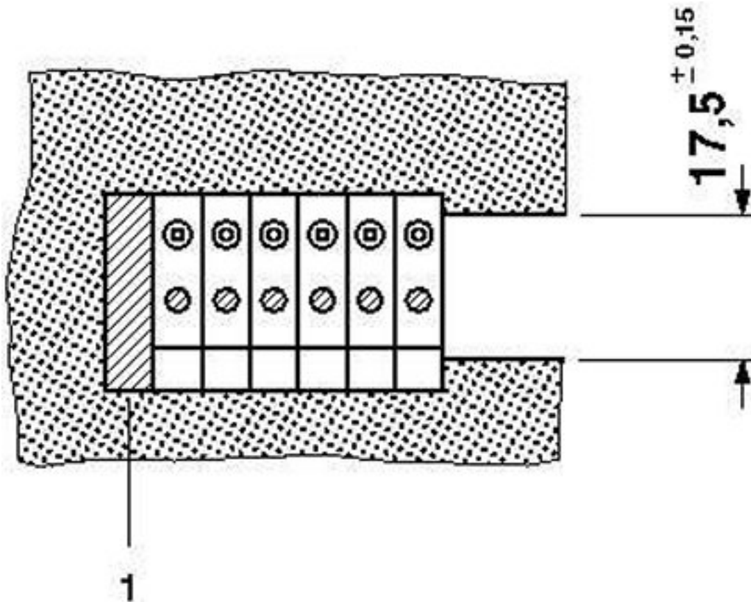
Dimensioned drawing
