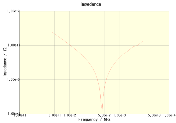
C1608C0G2A151J080AA
