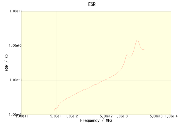
C1608C0G2A151J080AA
