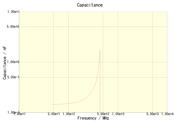
C1608C0G2A151J080AA
