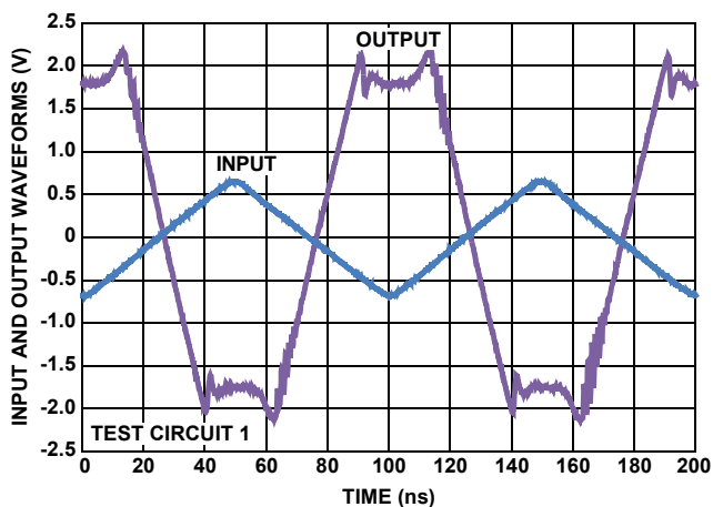
FIGURE 25. OVERDRIVE RECOVERY
