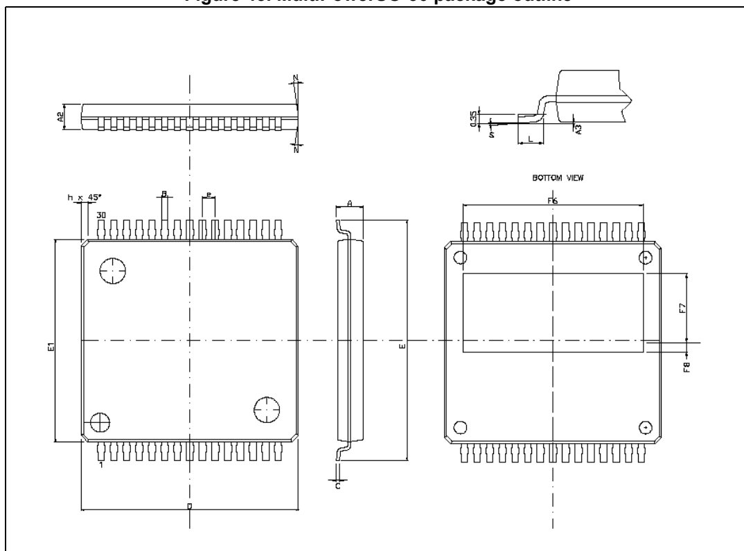
Figure 43. MultiPowerSO-30 package outline
