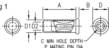
Fig 2 (Knockout bottom)
