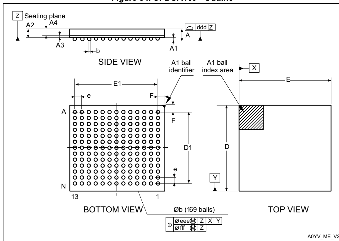
Figure 84. UFBGA169 - Outline
