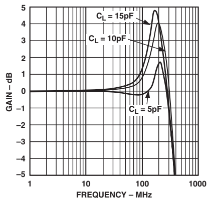
TPC 7. Small Signal Frequency Response for Various C_{LOAD} , V_{OUT} = 500 mV p-p, V_S = \pm 5 V, G = +1
