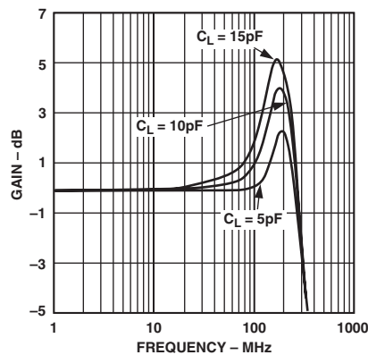
TPC 8. Small Signal Frequency Response for Various C_{LOAD} , V_{OUT} = 500 mV p-p, V_S = 5 V, G = +1
