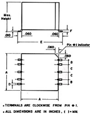
BOTTOM VIEW Larger size drawing
