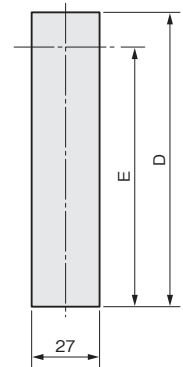
Layout of hole for installation
