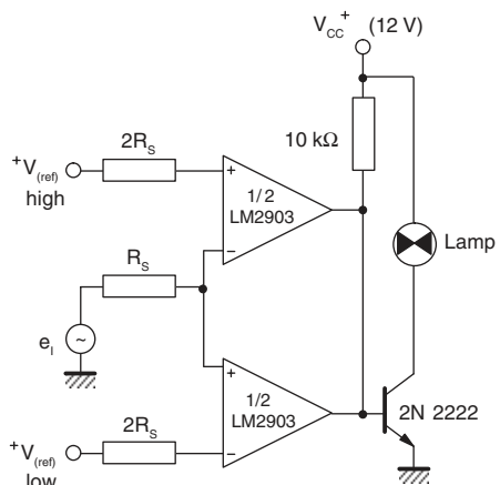
Figure 16. Limit comparator
