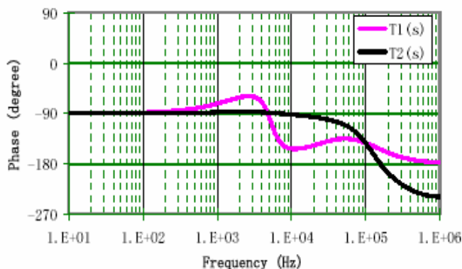
FIGURE 13. AN EXAMPLE OF ISL6261A COMPENSATION SPREADSHEET
