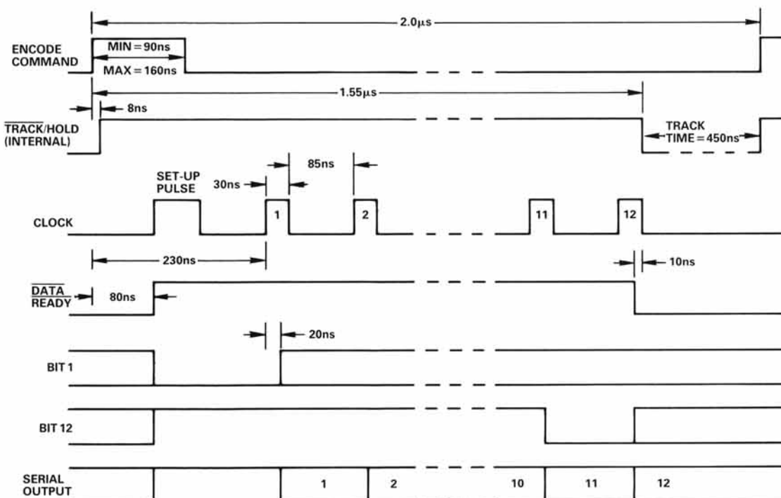
Figure 1. HAS-1204 Timing
