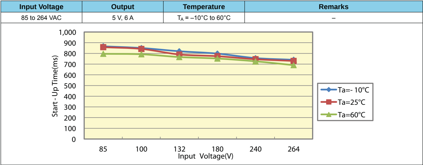
Figure 17. Start-Up Time (By Input Voltage)
