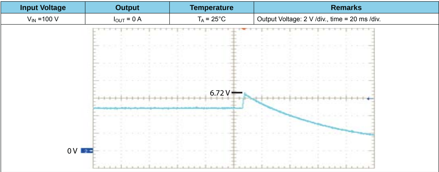
Figure 16. Overvoltage Protection Operation
