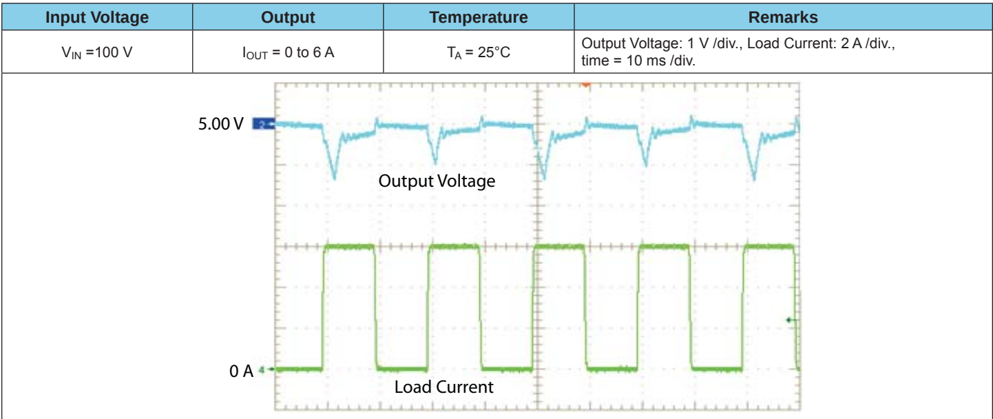
Figure 20. Dynamic Load
