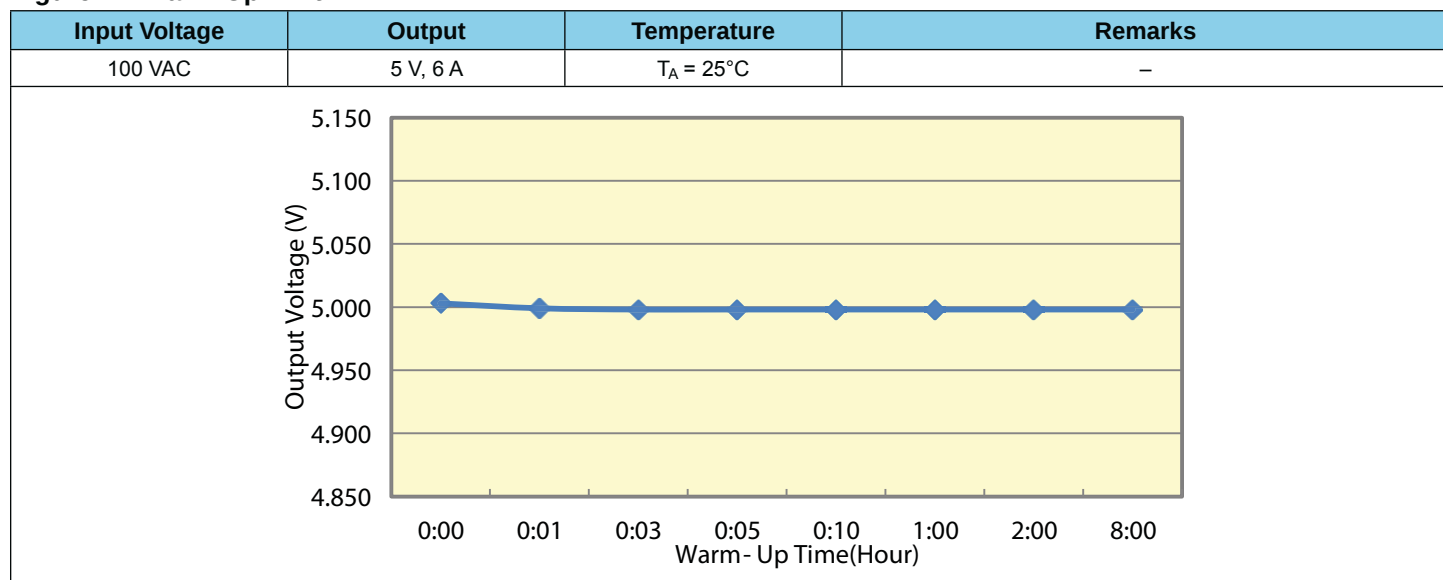
Figure 11. Warm-Up Drift
