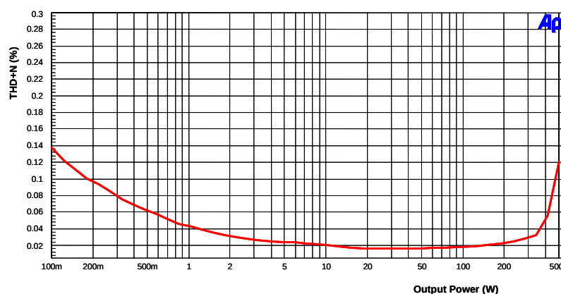
ZXCDSUBEV series THD+N versus power
