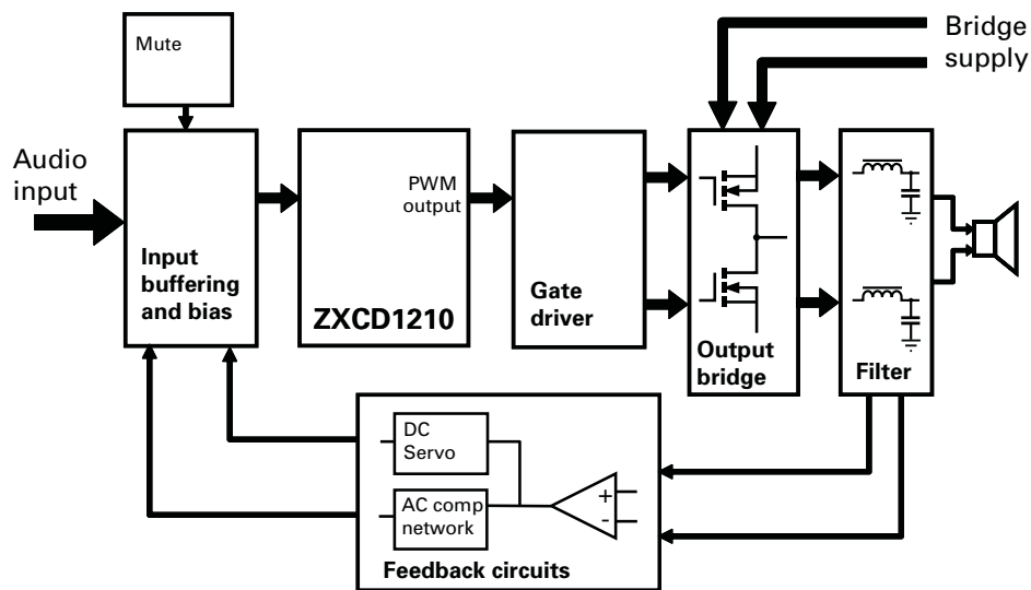
ZXCDSUBEV series architecture
