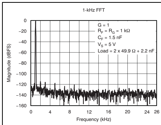
Figure 72. 1-kHz FFT
