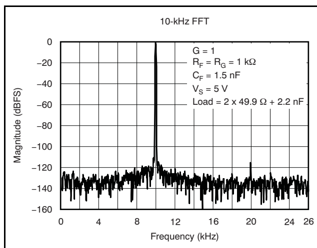
Figure 73. 10-kHz FFT
